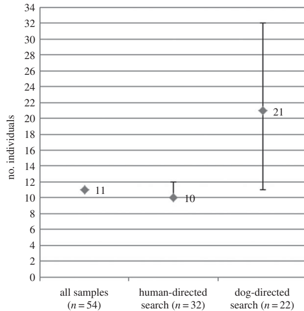
Figure 3. Kagwene population estimate using all genotyped samples, human-directed search samples only, and dog-directed search samples only (results were the same for all three grouping schemes). Error bars represent 95% confidence intervals.
