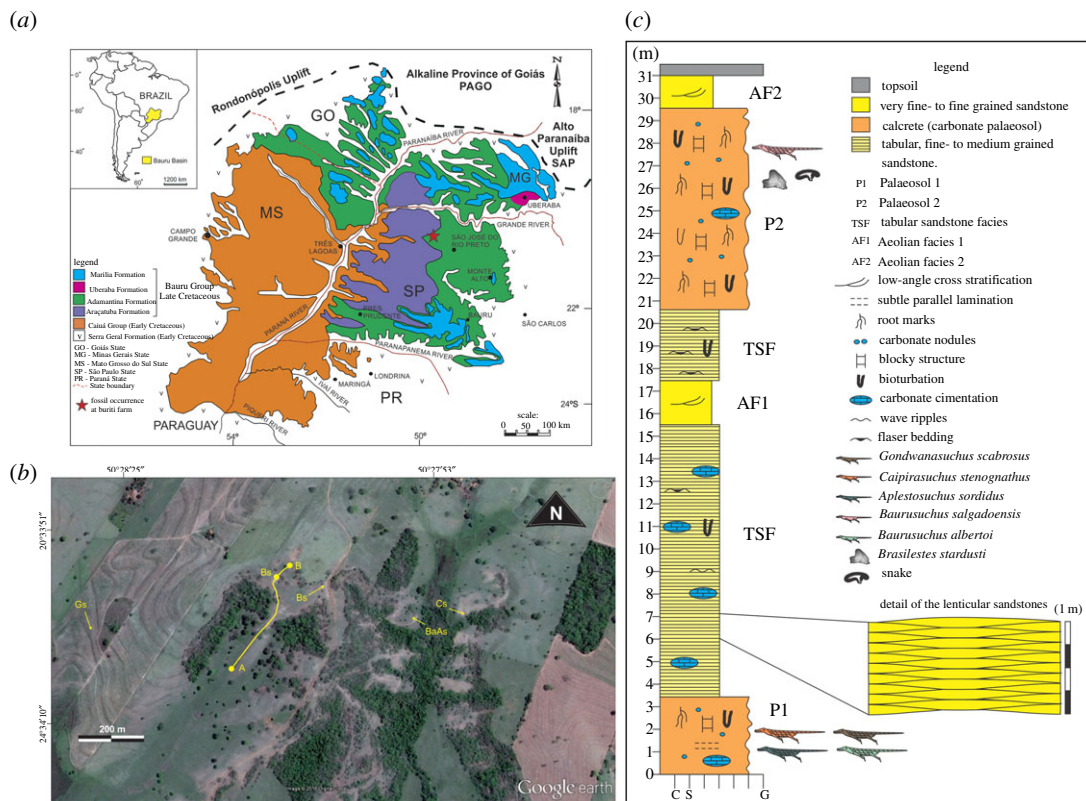
Figure 1. Geological settings. (a) Surface distribution map of Bauru Basin stratigraphic units (modified from ref. [17] using CoreDRAW 2017 www.coreldraw.com ); (b) Google Earth image (2016) marking fossil occurrences at Buriti Farm, São Paulo State, Brazil; (c) Stratigraphic column of the studied site. A–B, transect of the stratigraphic column; BaAs, Baurusuchus albertoi and Aplestosuchus sordidus type-locality; Bs (within the A–B transect), B. stardusti type-locality; Bs, Baurusuchus salgadoensis type-locality; Cs, Caipirasuchus stenognathus type-locality; Gs, Gondwanasuchus scabrosus type-locality.
